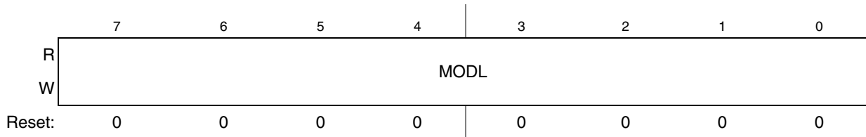
Figure 11-9. MTIM16 Modulo Register Low (MTIMMODL)
