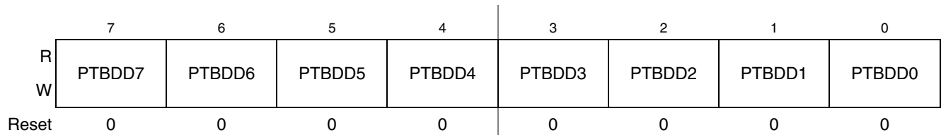
Figure 6-8. Data Direction for Port B Register (PTBDD)
