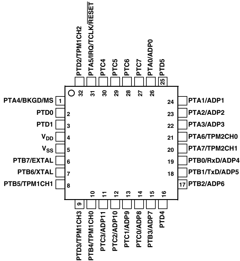
Figure 2-2. MC9S08FL16 Series 32-Pin LQFP Package
