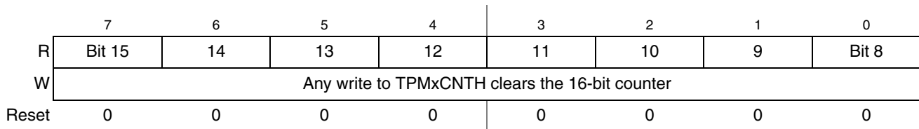
Figure 9-8. TPM Counter Register High (TPMxCNTH)
