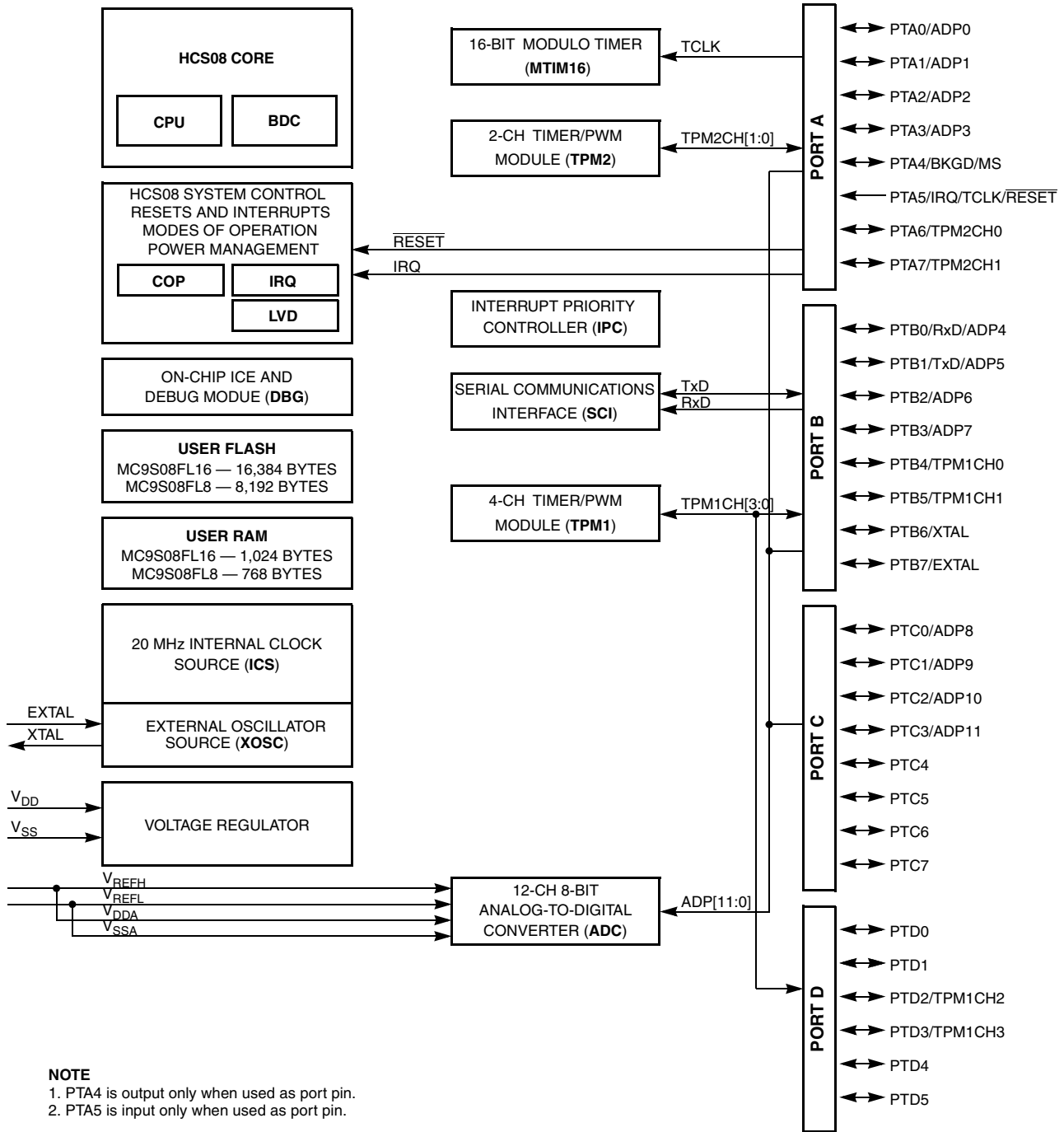
Figure 1-1. MC9S08FL16 Block Diagram
