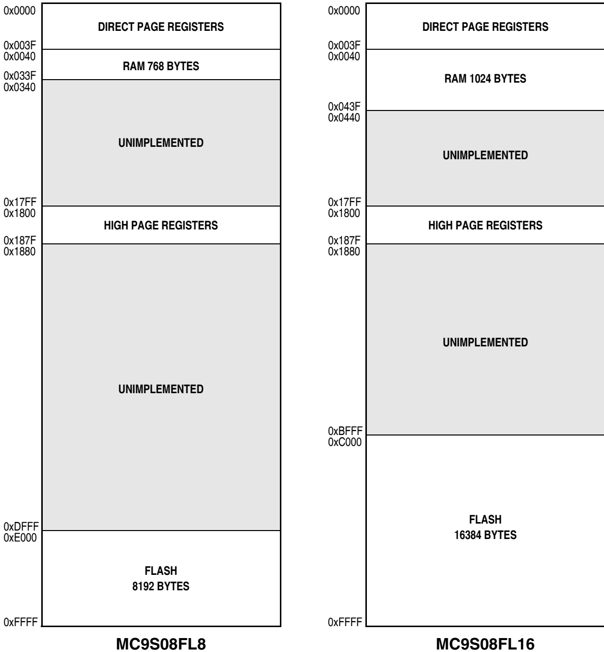
Figure 4-1. MC9S08FL16 Series Memory Map
