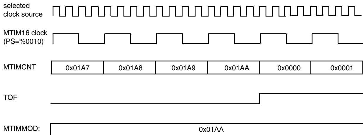
Figure 11-10. MTIM16 Counter Overflow Example
