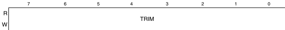
Figure 8-5. ICS Trim Register (ICSTRM)
