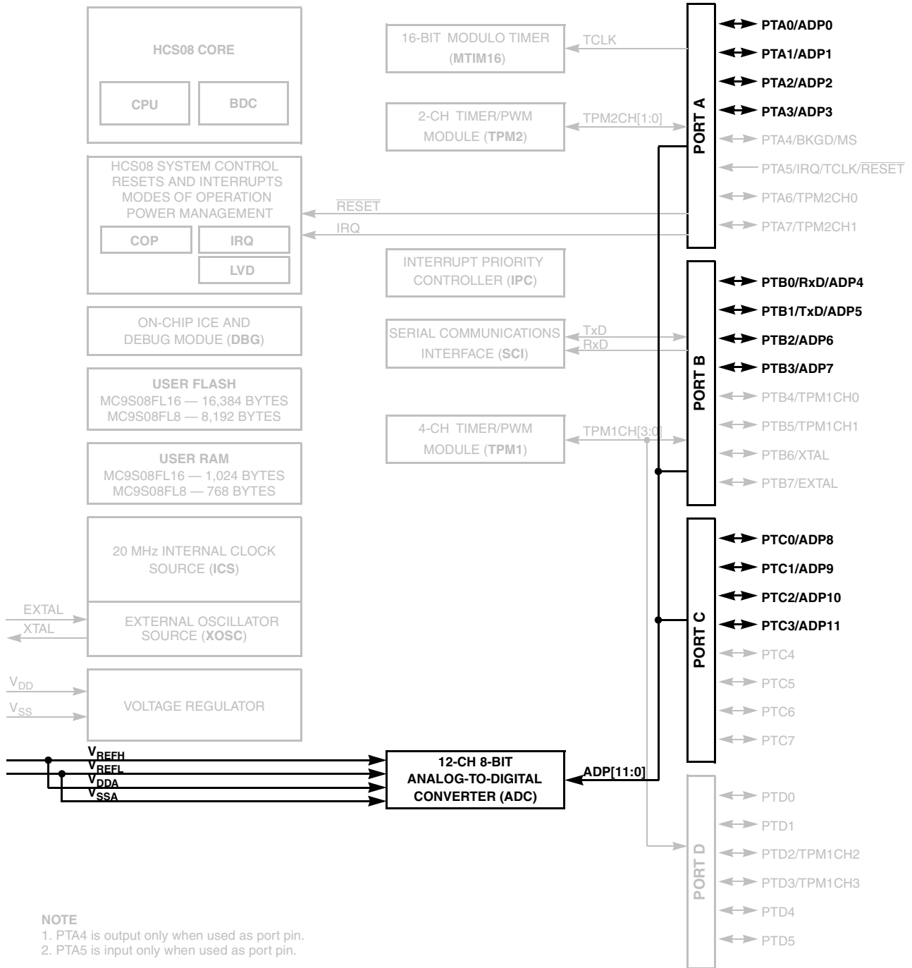
Figure 12-2. MC9S08FL16 Series Block Diagram Highlighting ADC Module and Pins.
