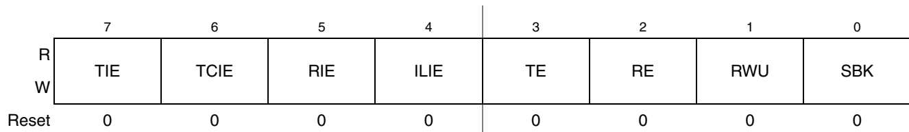
Figure 13-7. SCI Control Register 2 (SCIC2)
