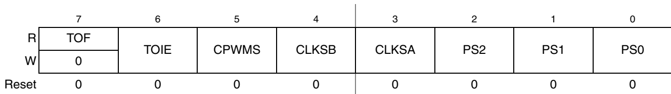
Figure 9-7. TPM Status and Control Register (TPMxSC)
