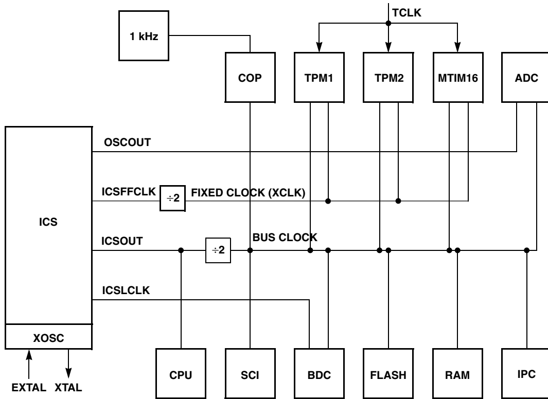
Figure 1-2. System Clock Distribution Diagram
