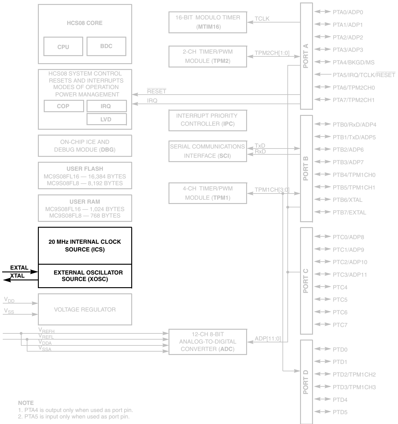
Figure 8-1. MC9S08FL16 Series Block Diagram Highlighting ICS Module and Pins
