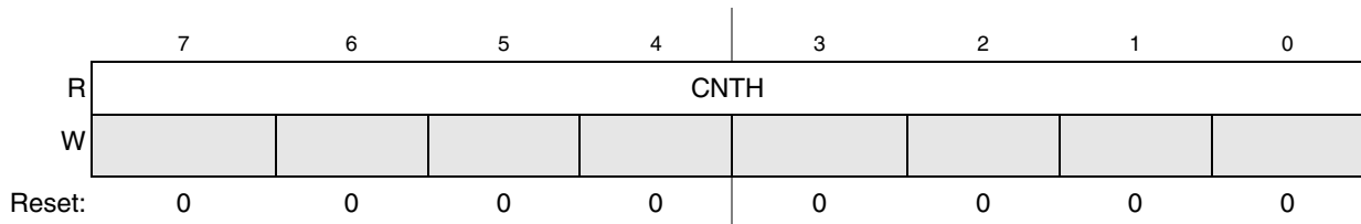
Figure 11-6. MTIM16 Counter Register High (MTIMCNTH)
