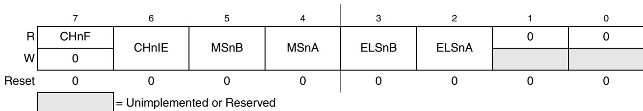
Figure 9-12. TPM Channel n Status and Control Register (TPMxCnSC)
