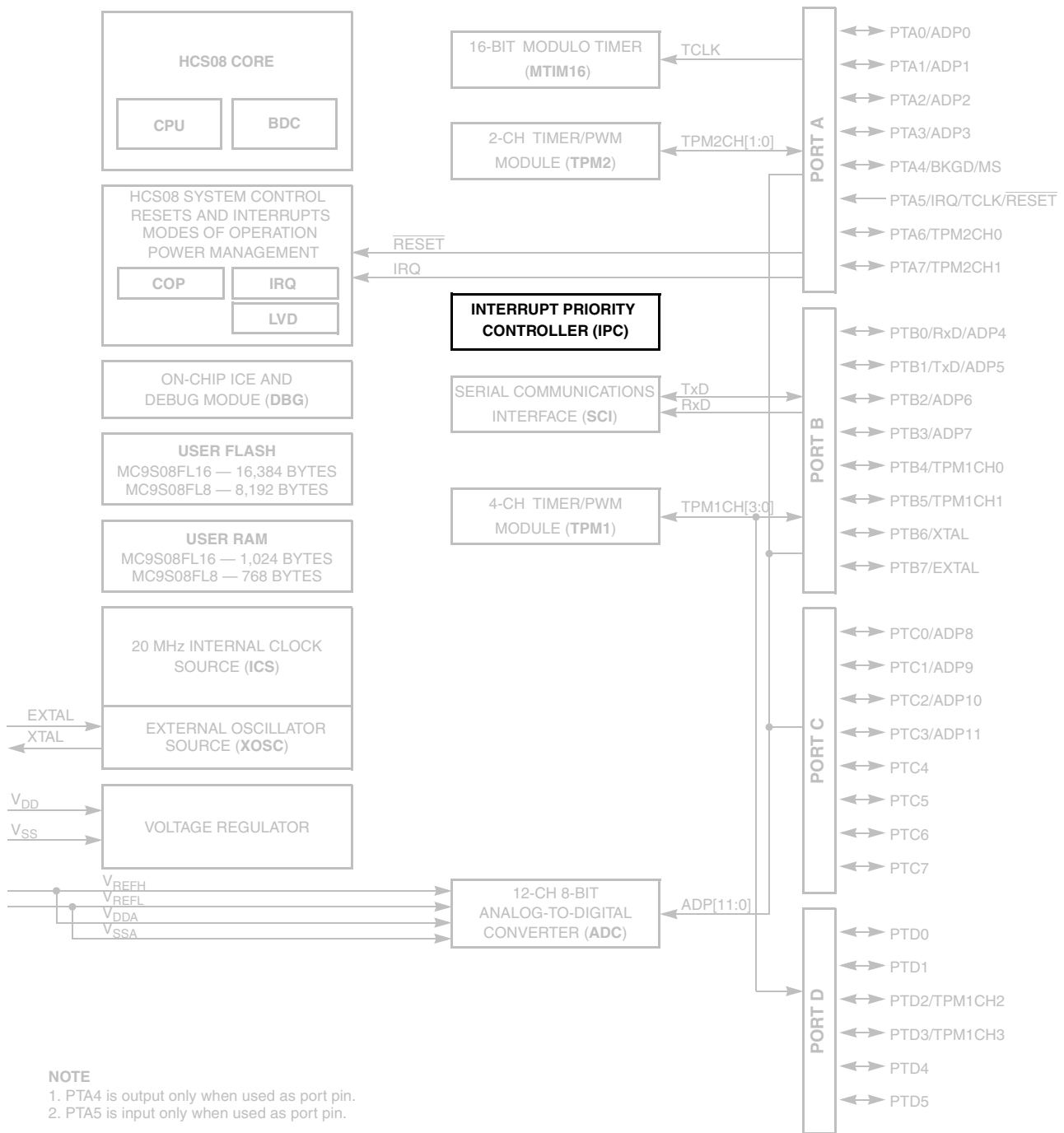
Figure 10-1. MC9S08FL16 Series Block Diagram Highlighting IPC Module
