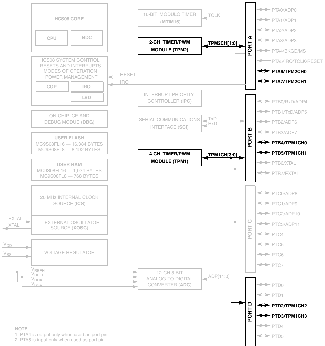
Figure 9-1. MC9S08FL16 Series Block Diagram Highlighting TPM Modules and Pins
