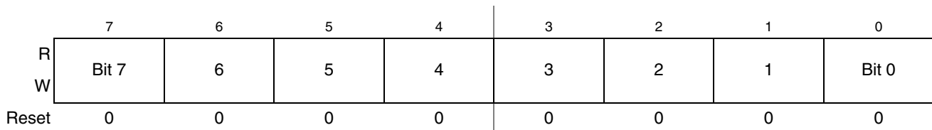
Figure 9-14. TPM Channel Value Register Low (TPMxCnVL)
