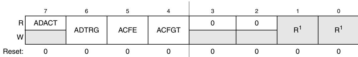
Figure 12-5. Status and Control Register 2 (ADCSC2)
