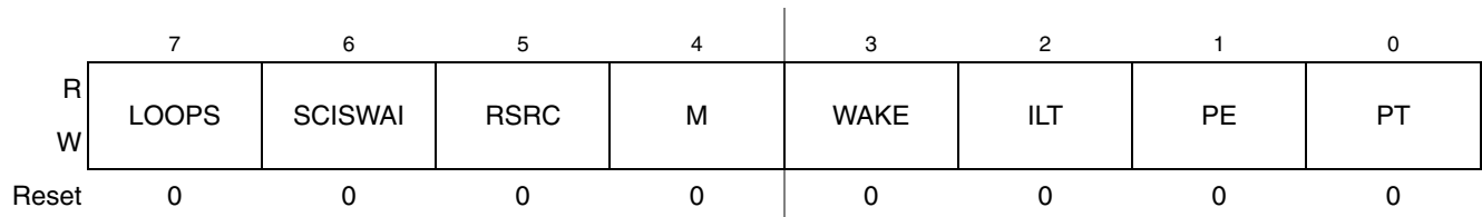
Figure 13-6. SCI Control Register 1 (SCIC1)
