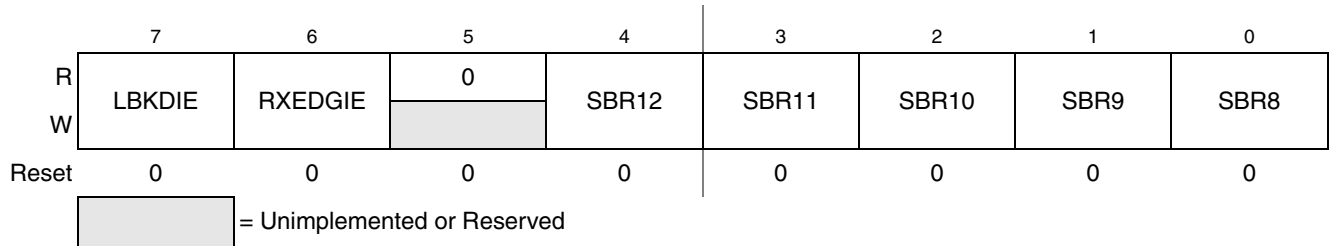
Figure 13-4. SCI Baud Rate Register (SCIBDH)
