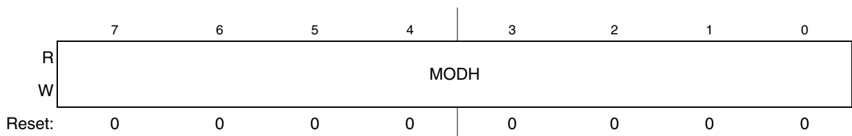
Figure 11-8. MTIM16 Modulo Register High (MTIMMODH)
