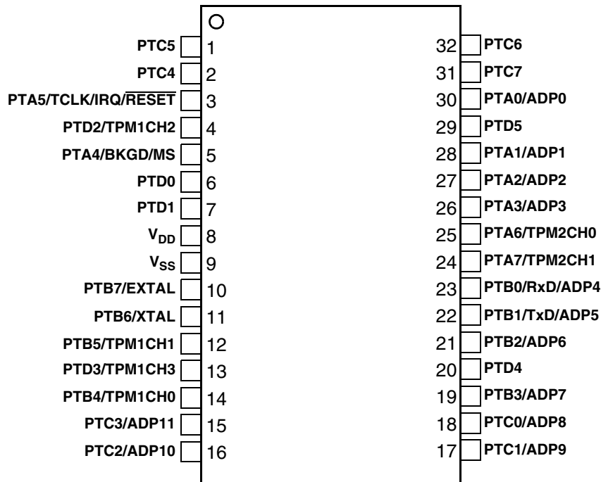
Figure 2-1. MC9S08FL16 Series 32-Pin SDIP Package
