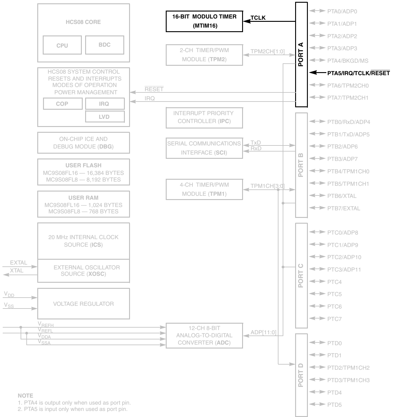
Figure 11-1. MC9S08FL16 Series Block Diagram Highlighting MTIM16 Module and Pin
