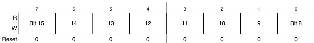
Figure 9-13. TPM Channel Value Register High (TPMxCnVH)
