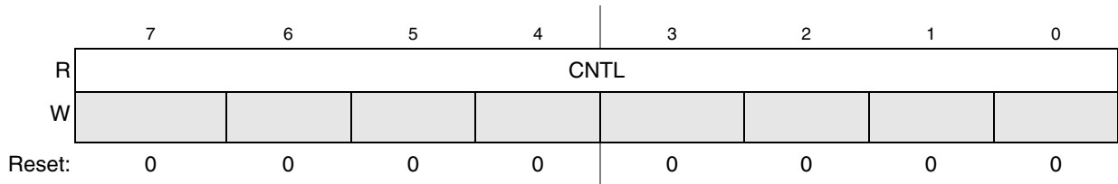
Figure 11-7. MTIM16 Counter Register Low (MTIMCNTL)
