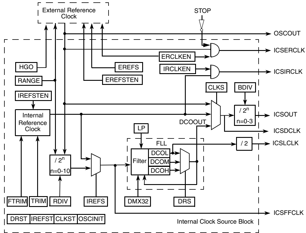
Figure 8-2. Internal Clock Source (ICS) Block Diagram
