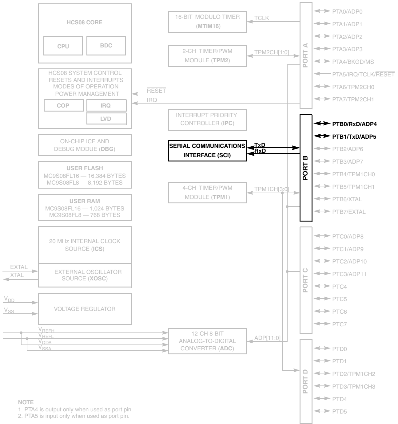
Figure 13-1. MC9S08FL16 Series Block Diagram Highlighting SCI Module and Pins
